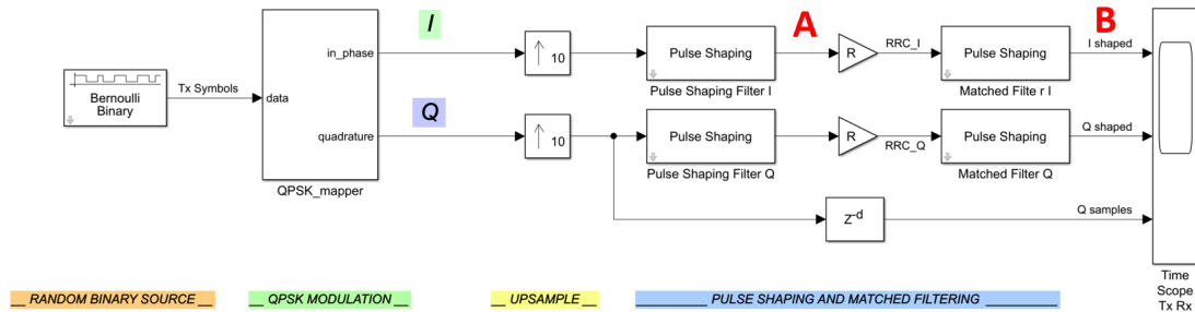
图 1 参考代码：/digital/simulation/pulse/RRC_matched.slx
