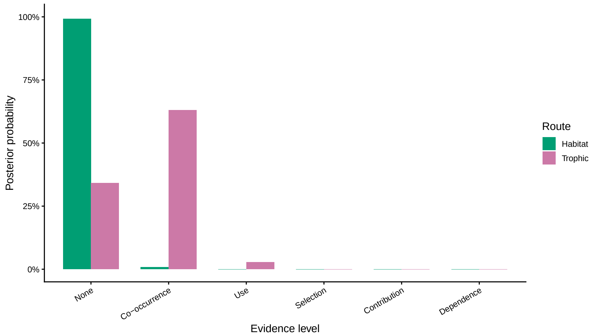
Evidence-level probabilities for Pachymetopon blochii
