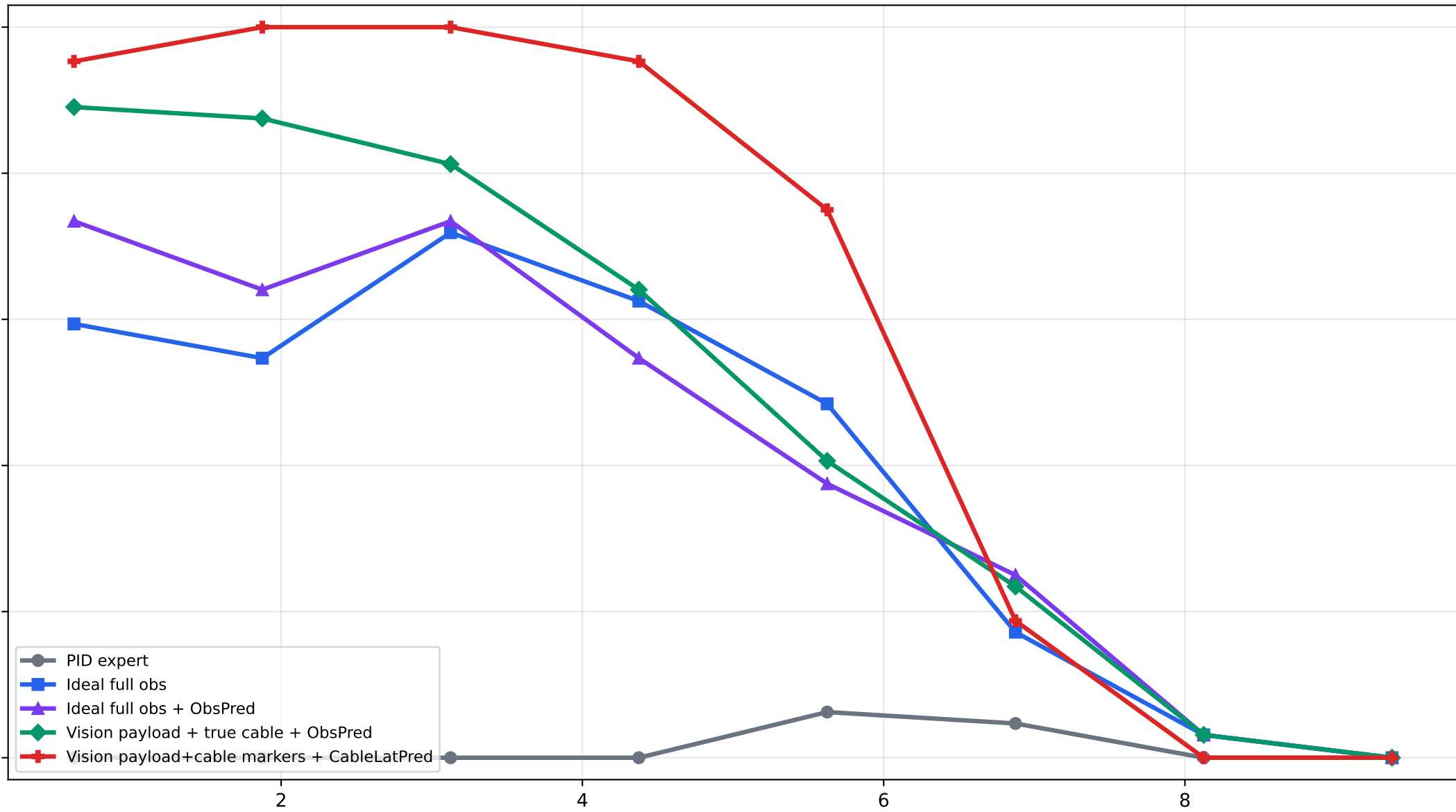
Strict Success Rate by Wind Speed
