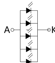
Backlight Circuit Diagram: (背光电路图)
