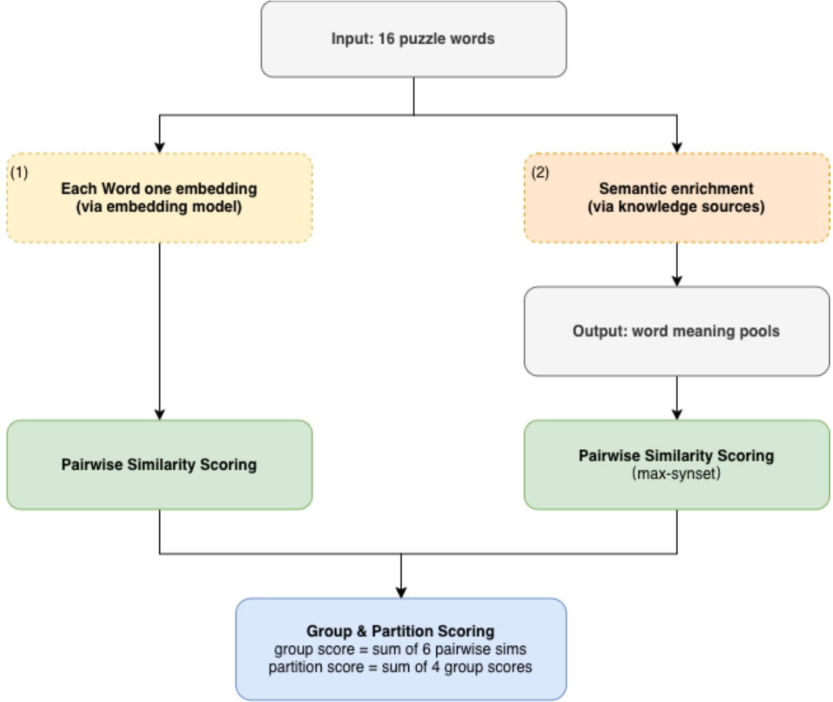
Figure 5.1: The two configurations of the scoring function compared in this thesis. Dashed borders mark the points where configurations differ; solid borders mark stages that are the same throughout. Configuration (1) embeds each word directly. Configuration (2) expands each word into a pool of meanings first, and then take the maximum over all pairs of meanings as the single similarity.
