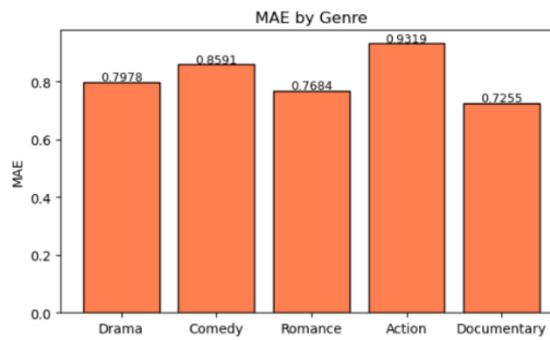
Fairness Analysis — Genre
