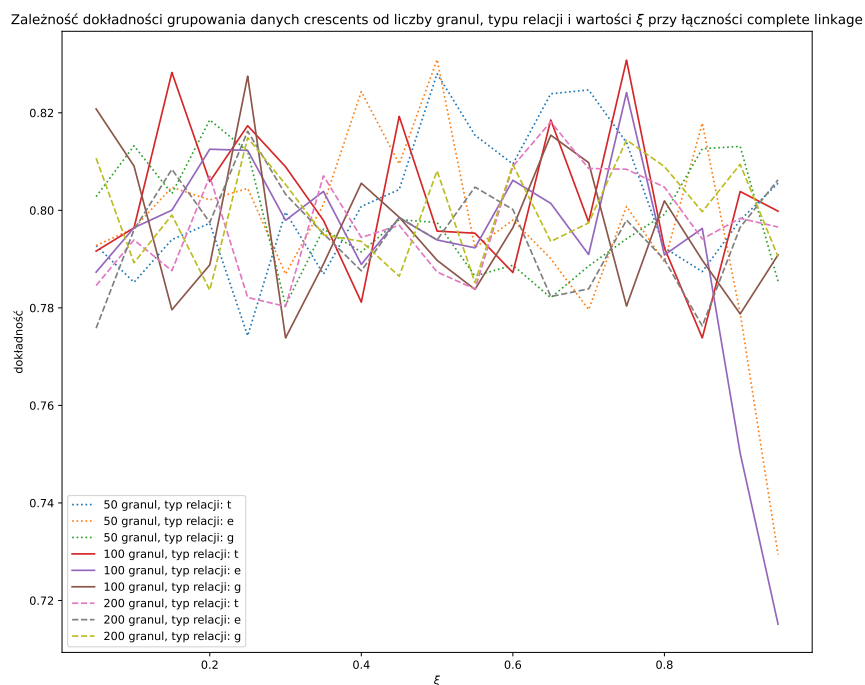
(b) COMPLETELINKAGE
