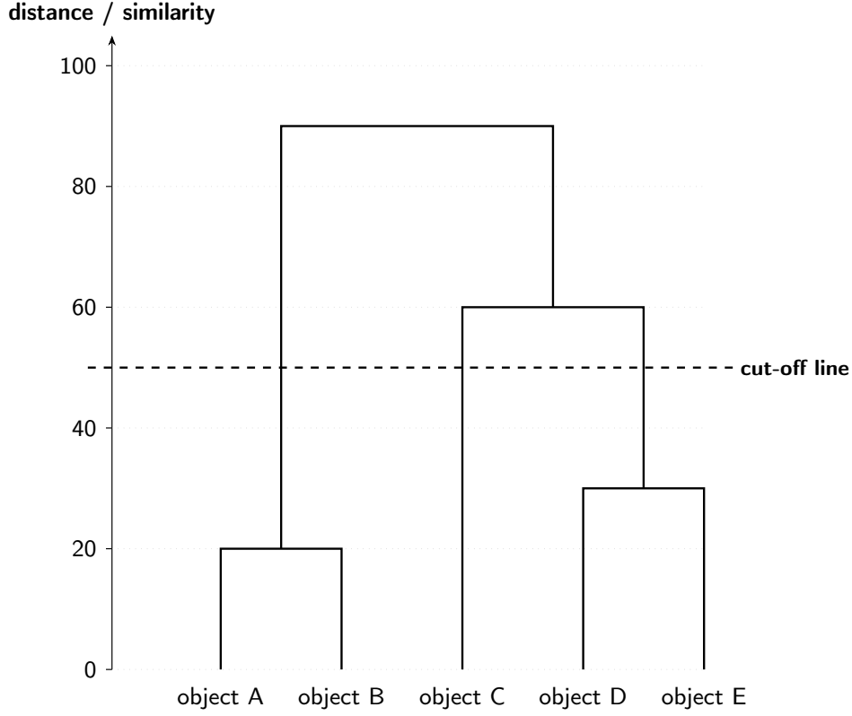
Figure 1: Example of a dendrogram for hierarchical clustering of five objects with a cut-off line at distance 50.
