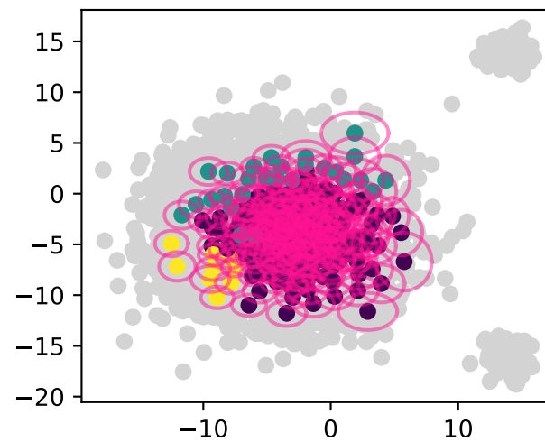
-10 0 10 200 granul, \xi = 0.9
