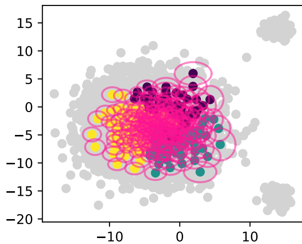
-10 0 10 200 granul, \xi = 0.5
