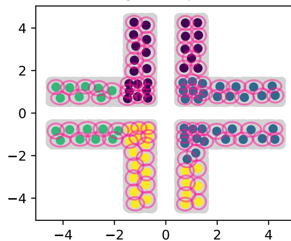
200 granul, \xi = 0.9
