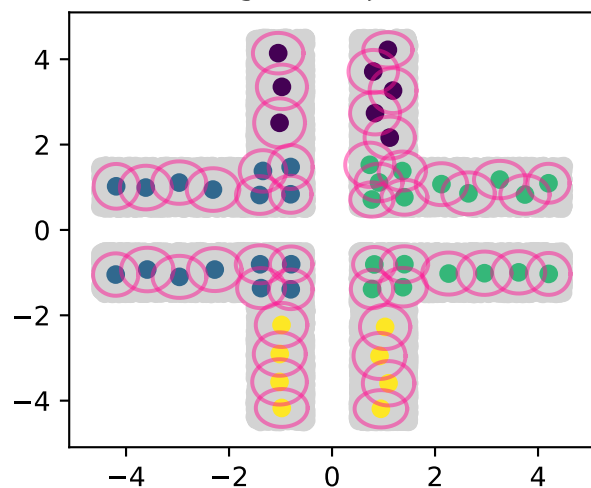
100 granul, \xi = 0.5
