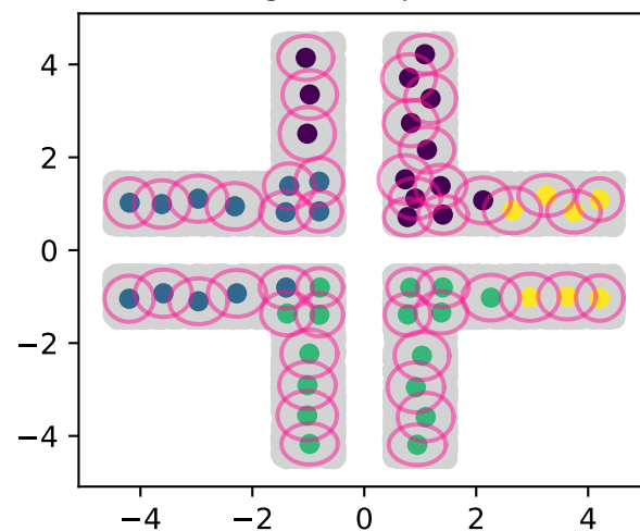
100 granul, \xi = 0.9
