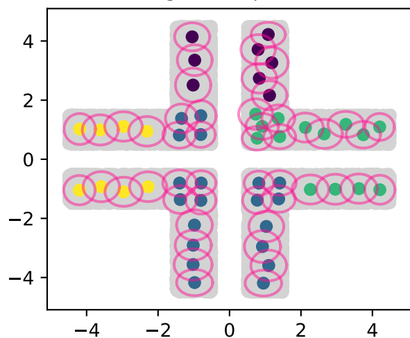
100 granul, \xi = 0.1
