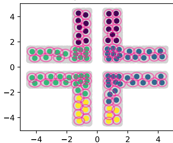
200 granul, \xi = 0.5
