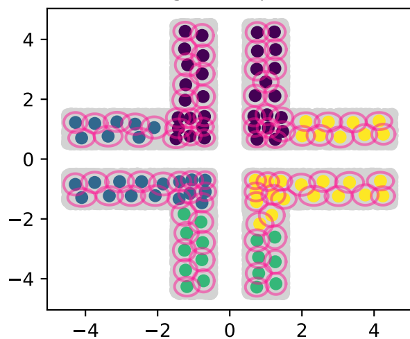
200 granul, \xi = 0.1
