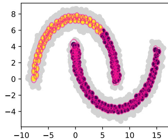
200 granul, \xi = 0.9
