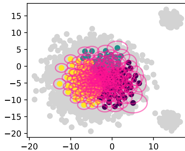
200 granul, \xi = 0.9
