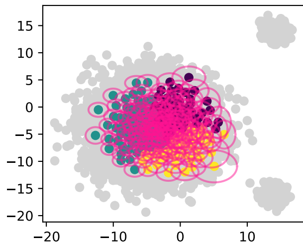
200 granul, \xi = 0.1
