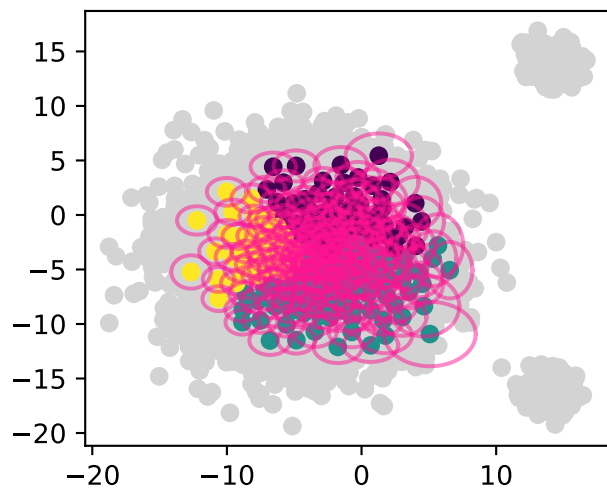
200 granul, \xi = 0.5
