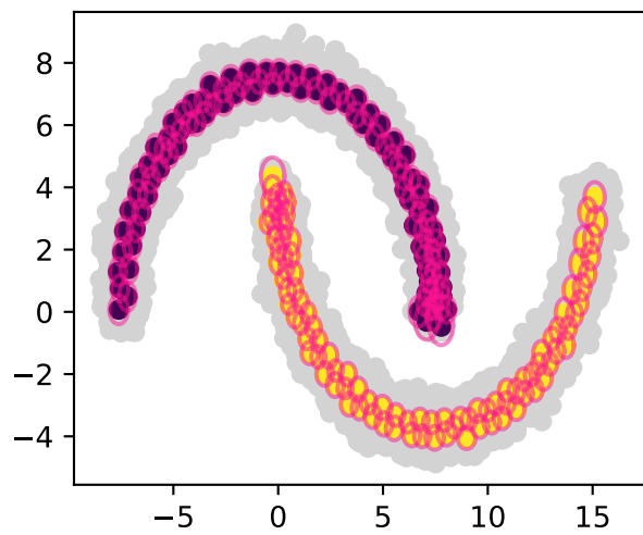
200 granul, \xi = 0.1
