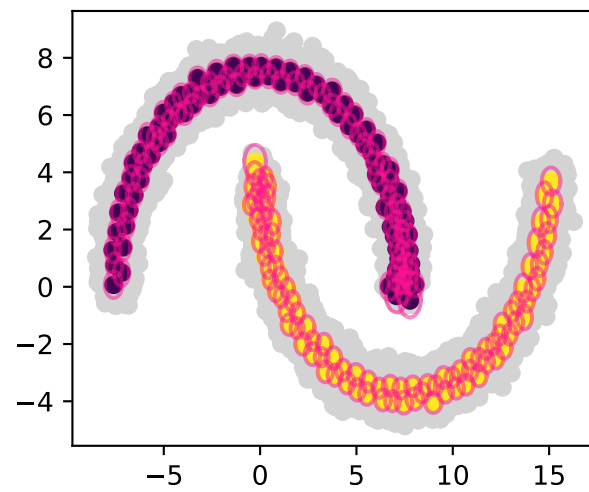
200 granul, \xi = 0.9
