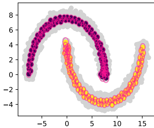
200 granul, \xi = 0.5
