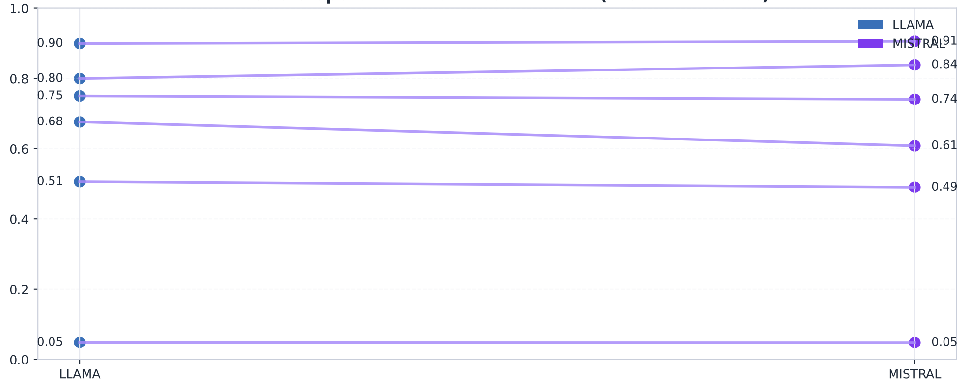
RAGAS Slope Chart — UNANSWERABLE (LLaMA → Mistral)
