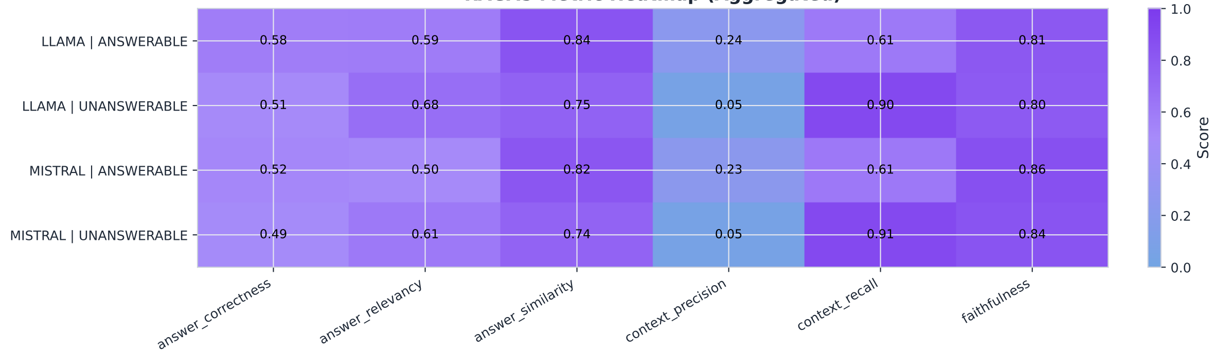
RAGAS Metric Heatmap (Aggregated)
