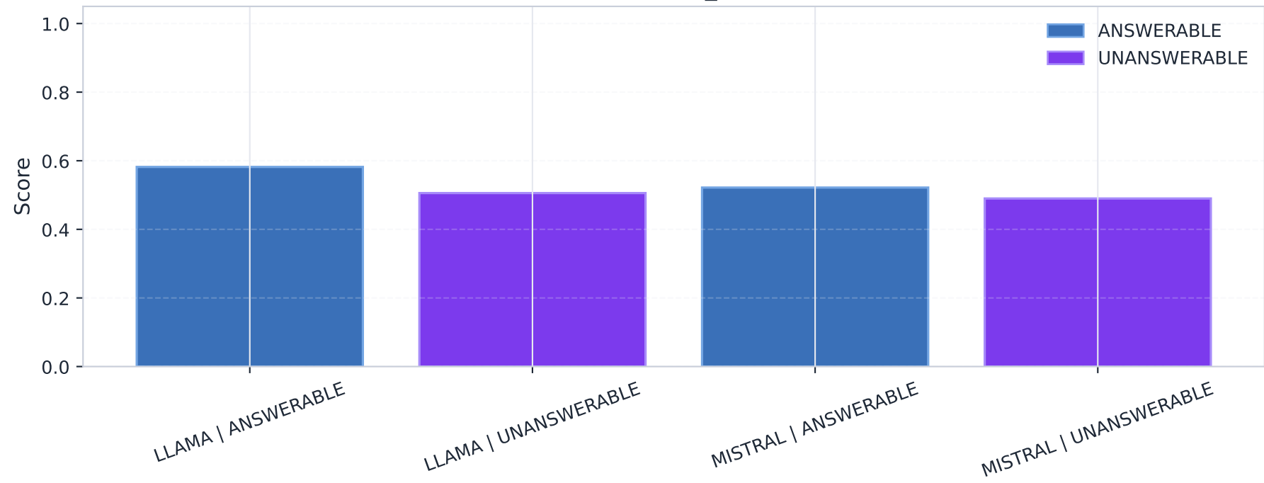
RAGAS — answer_correctness
