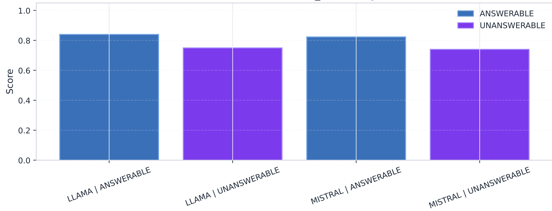
RAGAS — answer_similarity
