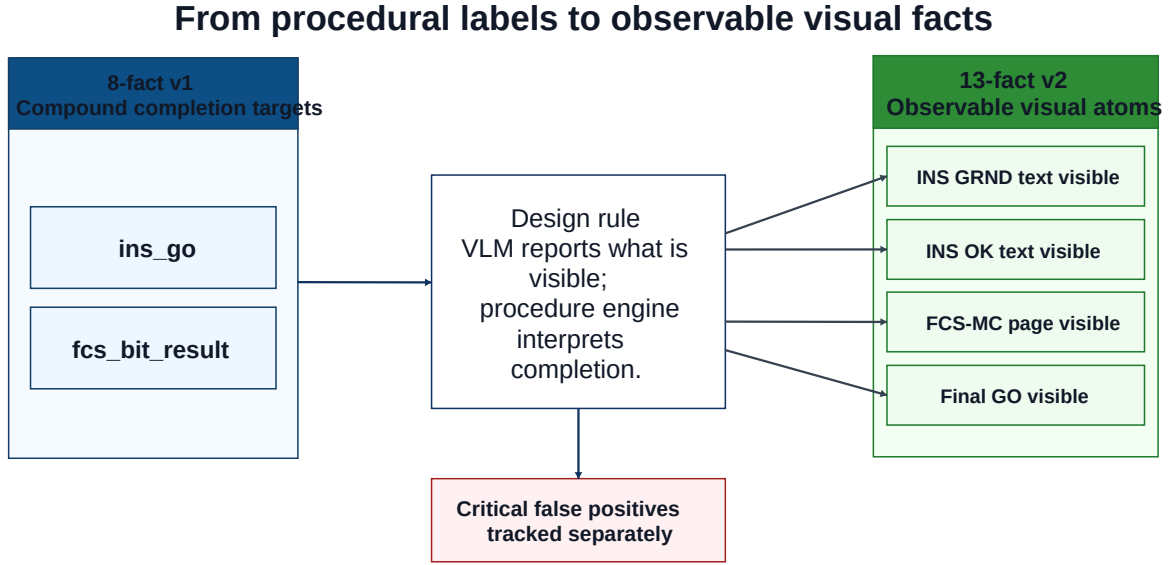
Figure 4.2: Ontology evolution from 8-fact v1 to 13-fact v2. Compound targets such as ins_go and broad FCS-MC completion facts were decomposed into locally verifiable visual atoms; the procedure engine then combines those observations with telemetry, phase, and timing evidence.
