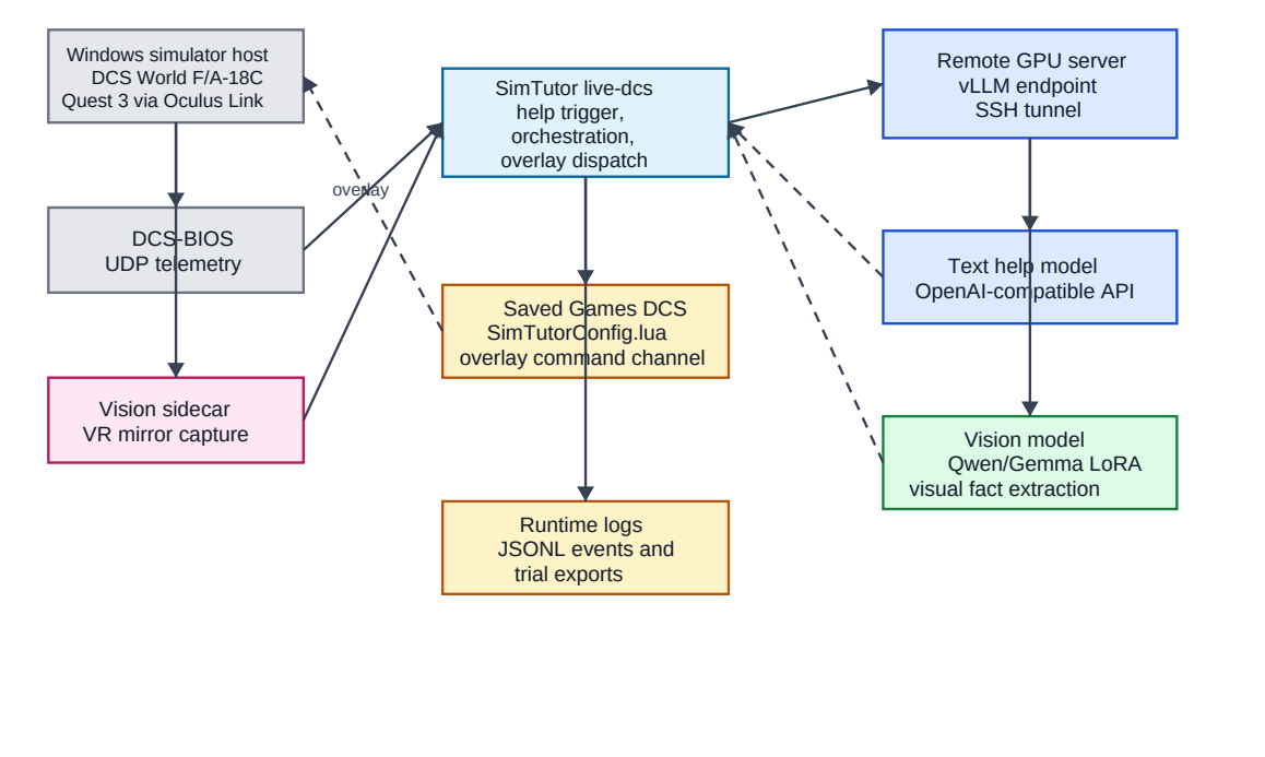
Deployment topology
