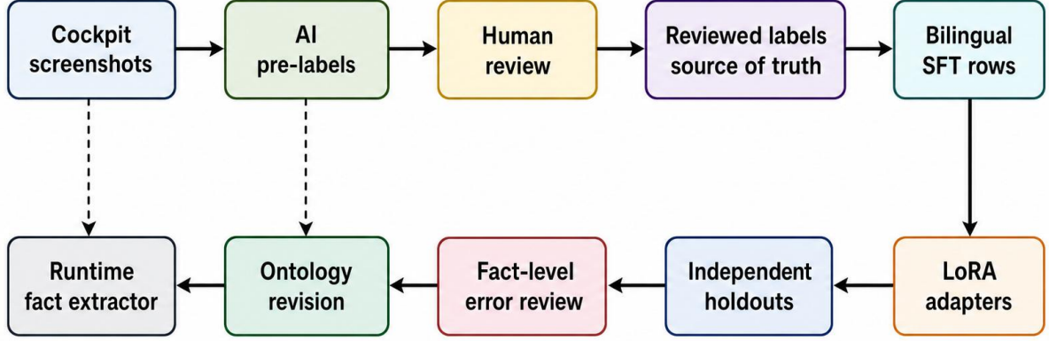
Figure 4.1: VLM adaptation pipeline. DCS World composite screenshots are pre-labelled, human-reviewed, converted into bilingual supervised fine-tuning rows, adapted with LoRA, evaluated on independent holdout sets, and used to drive ontology revision.
