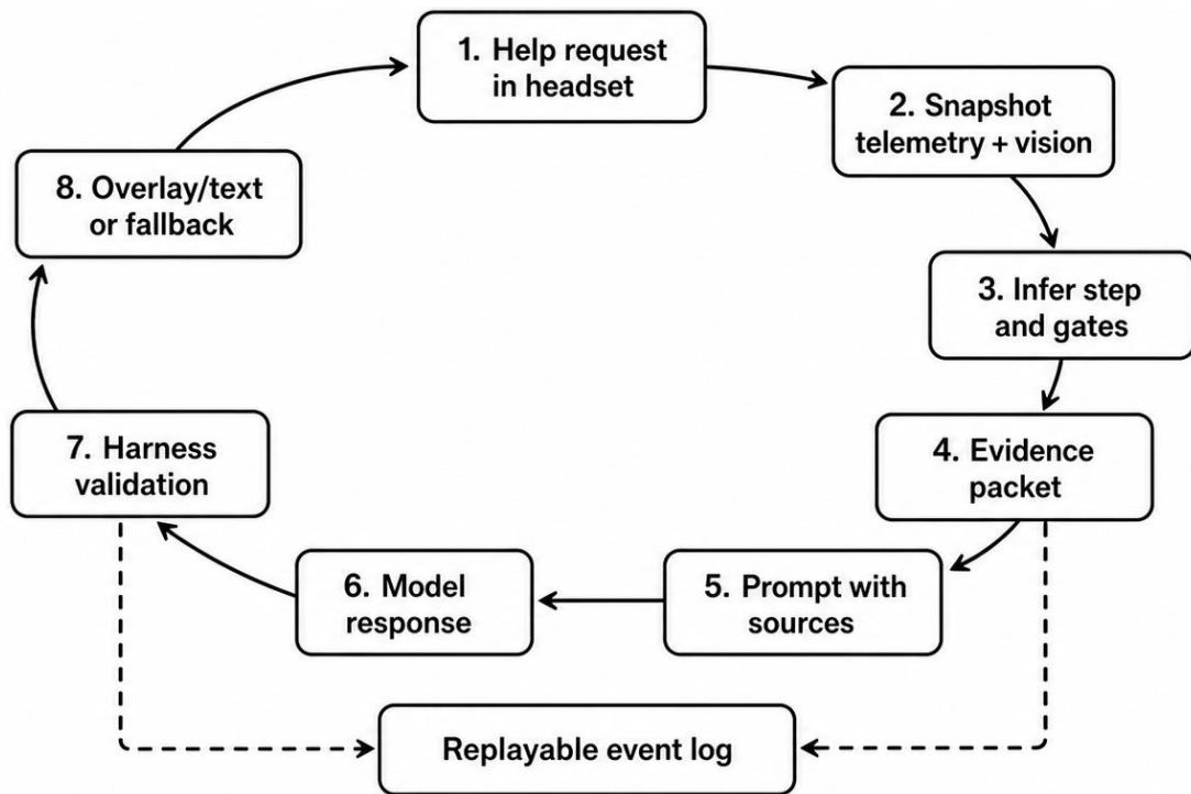
Figure 3.3: Live evidence-grounded help cycle. Assistance begins with an observation snapshot, turns it into an evidence packet, asks the model for a structured response, validates the result, and logs the displayed output.
