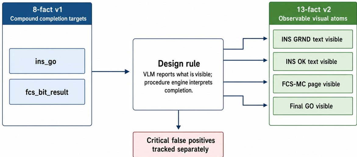
Figure 4.2: Ontology evolution from 8-fact v1 to 13-fact v2. Compound targets such as ins_go and broad FCS-MC completion facts were decomposed into locally verifiable visual atoms; the procedure engine then combines those observations with telemetry, phase, and timing evidence.
