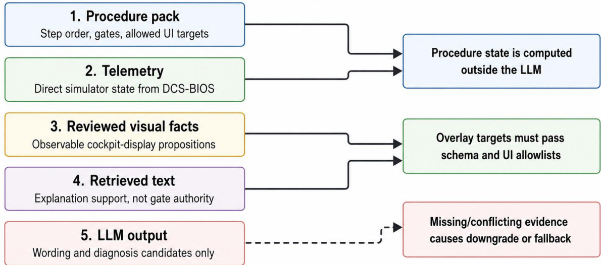
Figure 3.2: Authority boundaries for grounded tutoring. Procedure rules and telemetry constrain state; reviewed visual facts provide bounded display evidence; retrieval and LLM output support explanation but do not override gates or UI allowlists.
