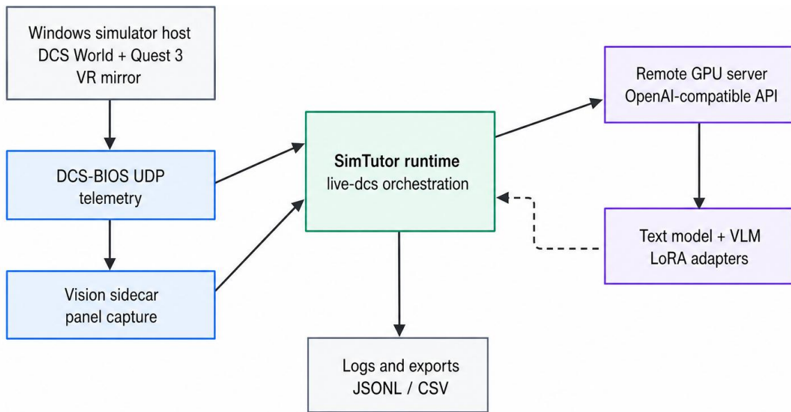
Figure 9.2: Deployment topology used by the prototype. The simulator, Quest 3 overlay path, local runtime, replay utilities, and remote model providers are separated so that live trials and offline analysis can use the same evidence and logging contracts.
