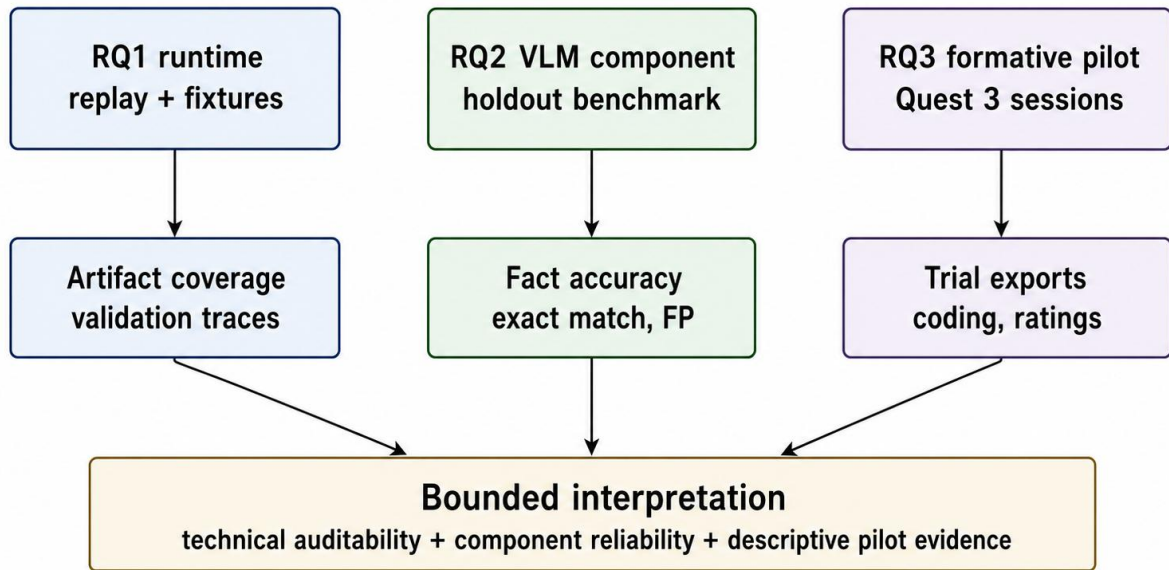
Figure 6.1: Evaluation and data flow across research questions. Replay and harness artifacts support RQ1, VLM benchmark artifacts support RQ2, and Quest 3 pilot exports support RQ3 descriptive findings.
