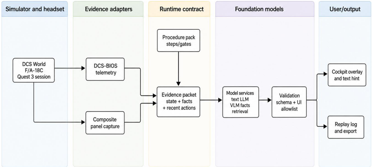
Figure 3.1: Evidence-grounded SimTutor architecture. Simulator observations, authored procedure rules, foundation-model outputs, and user-facing overlay actions are separated by explicit runtime contracts.
