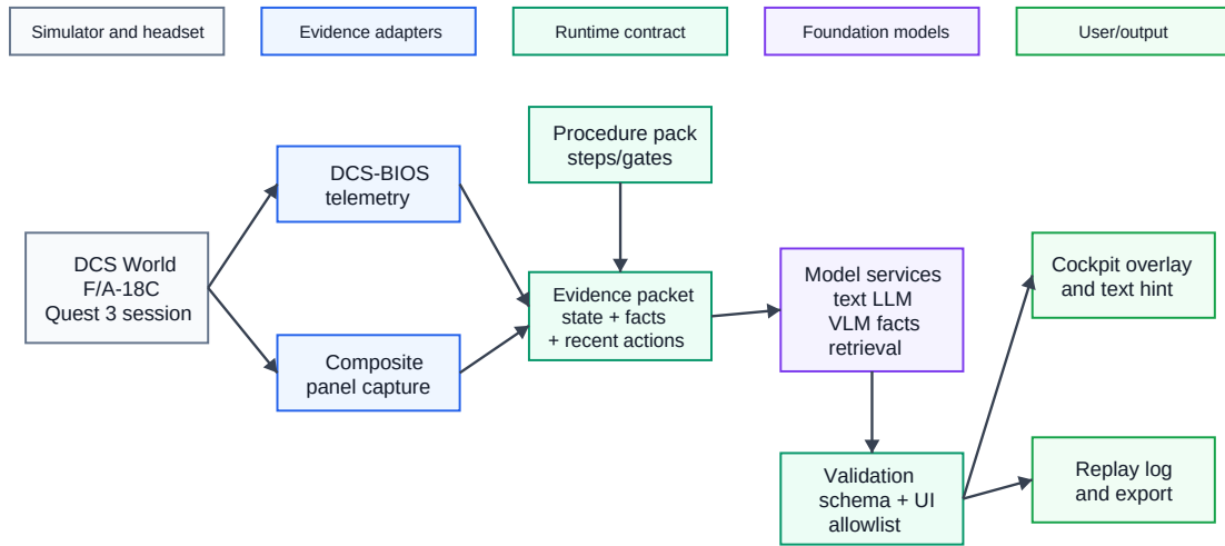
Evidence-grounded SimTutor architecture
