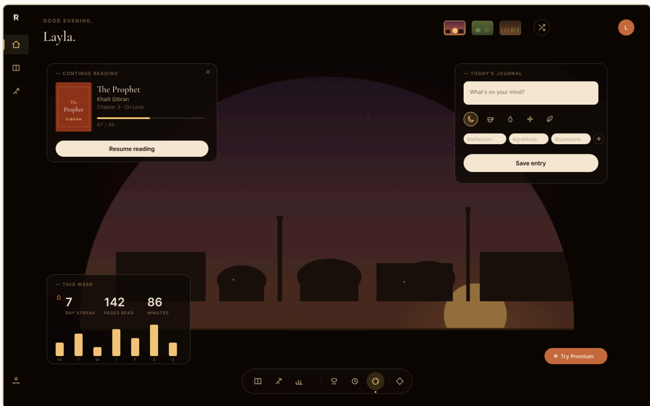
03 — Dashboard
