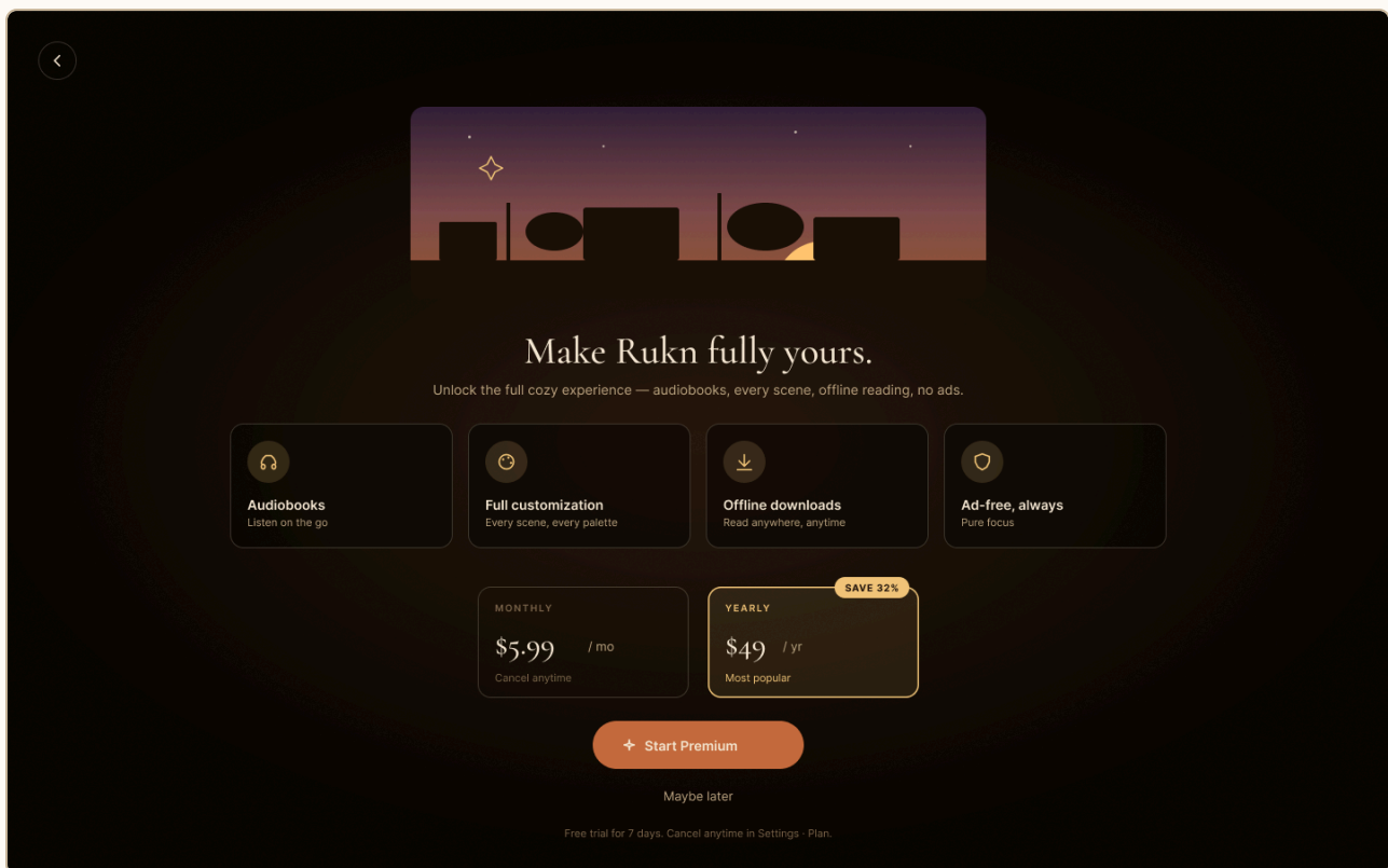
08 — Premium upgrade
