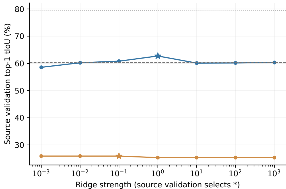
HC-STVG-v2
