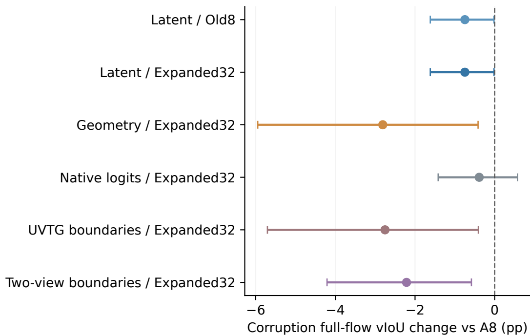
HC-STVG-v2 — confirmation
