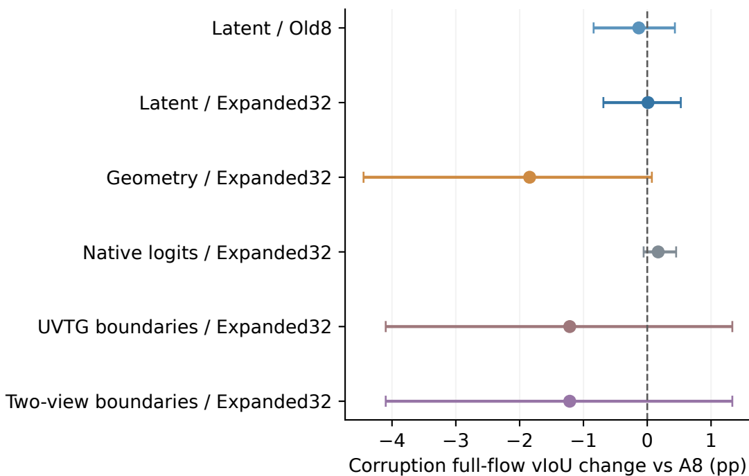
VidSTG — confirmation
