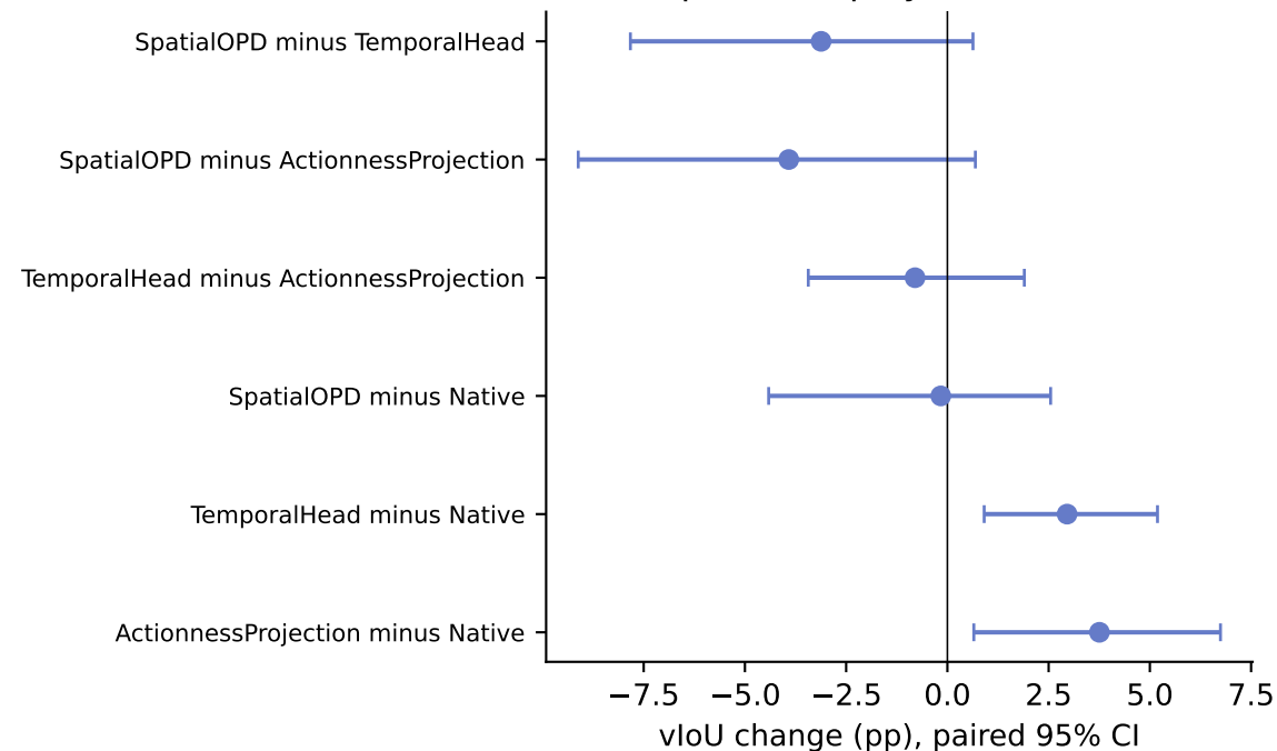
hc2 paired deployment contrasts
