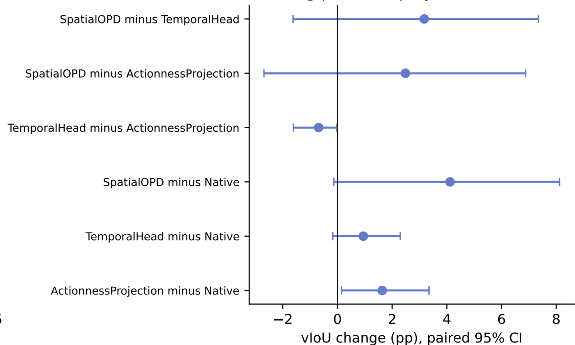
vidstg paired deployment contrasts
