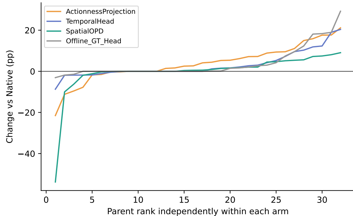
vidstg vIoU complete parent effects
