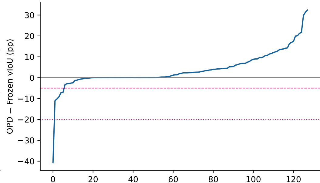
VidSTG target: all 128 parent effects
