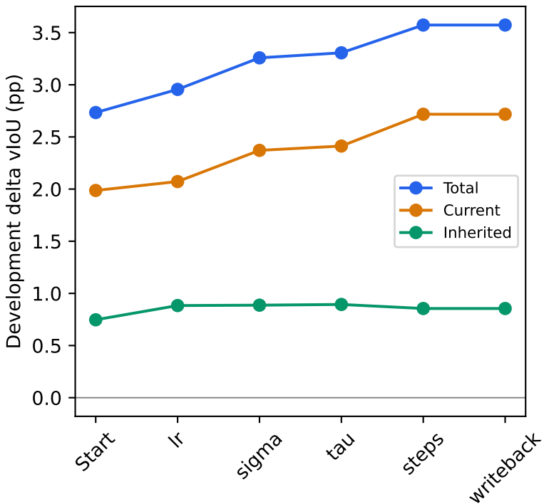
Greedy locking, complete negative tail, and real adaptation cost (development selection)
