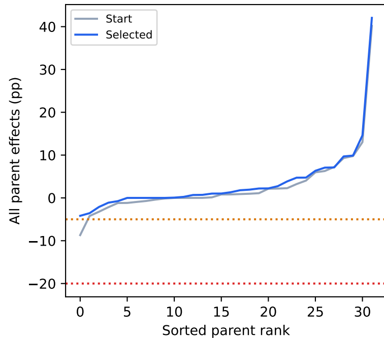
Greedy locking, complete negative tail, and real adaptation cost (development selection)
