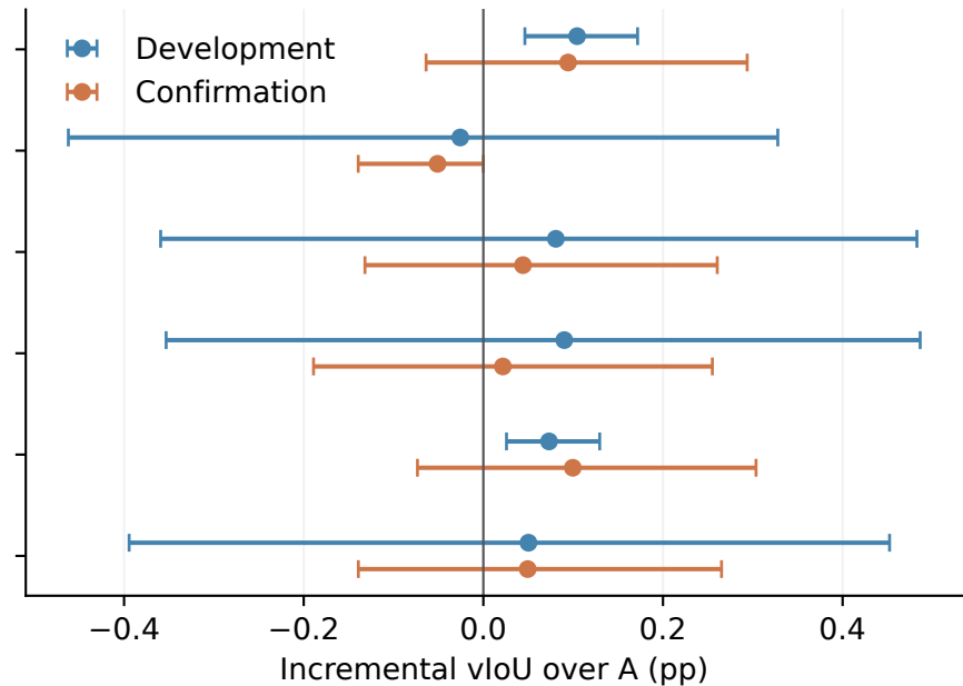
HC-STVG-v2
