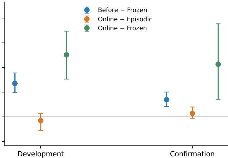
HC-STVG-v2
