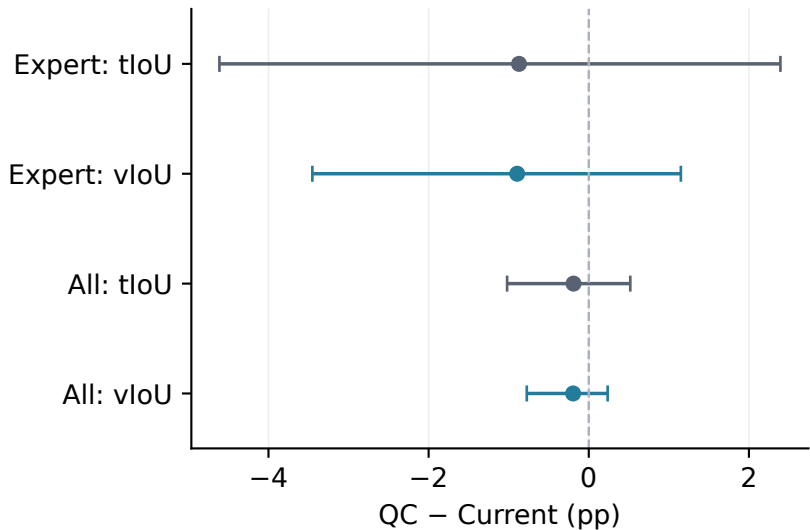
HC-STVG-v2
