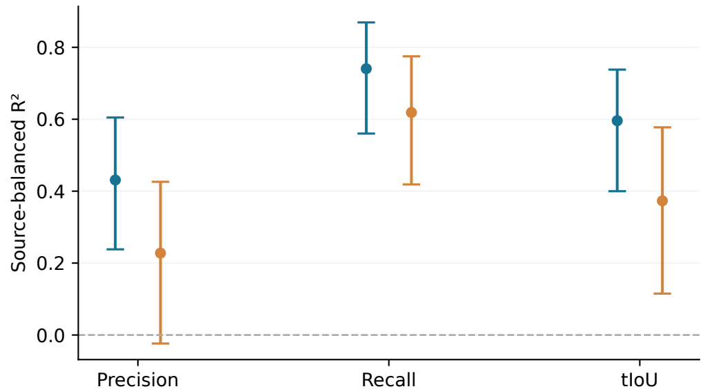
HC-STVG-v2
