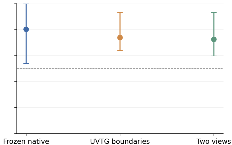
HC-STVG-v2
