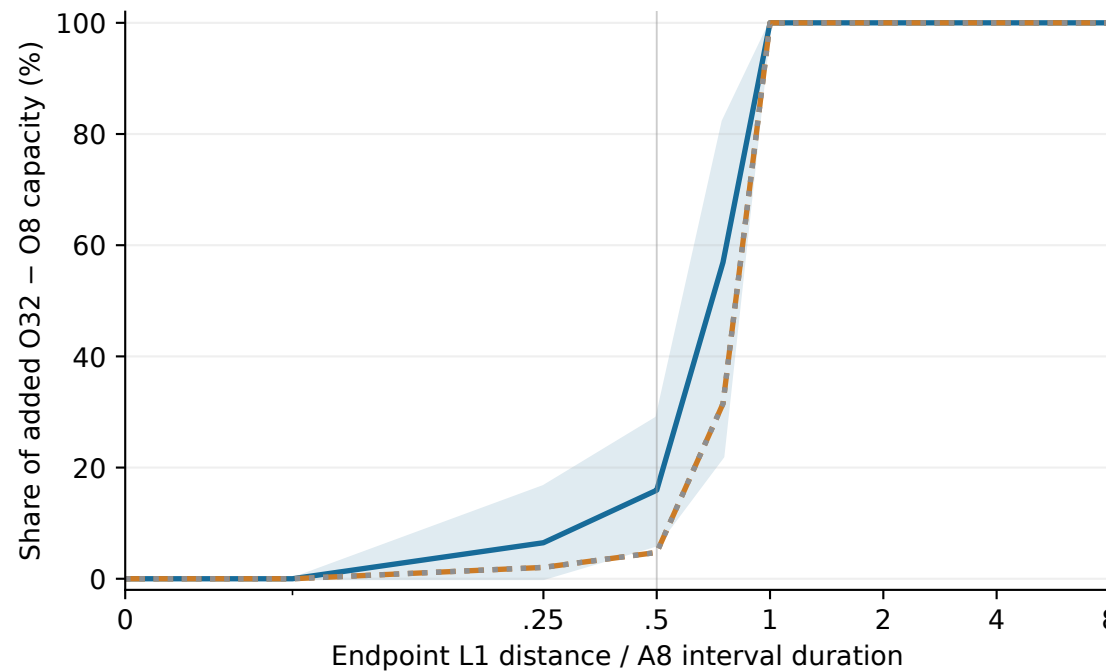
VidSTG/confirmation
