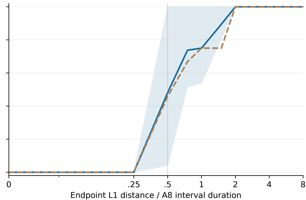
HC-STVG-v2/confirmation
