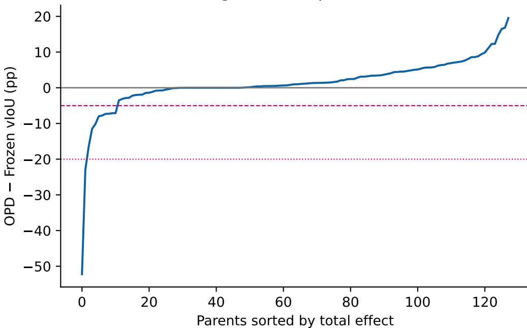
HC2 target: all 128 parent effects
