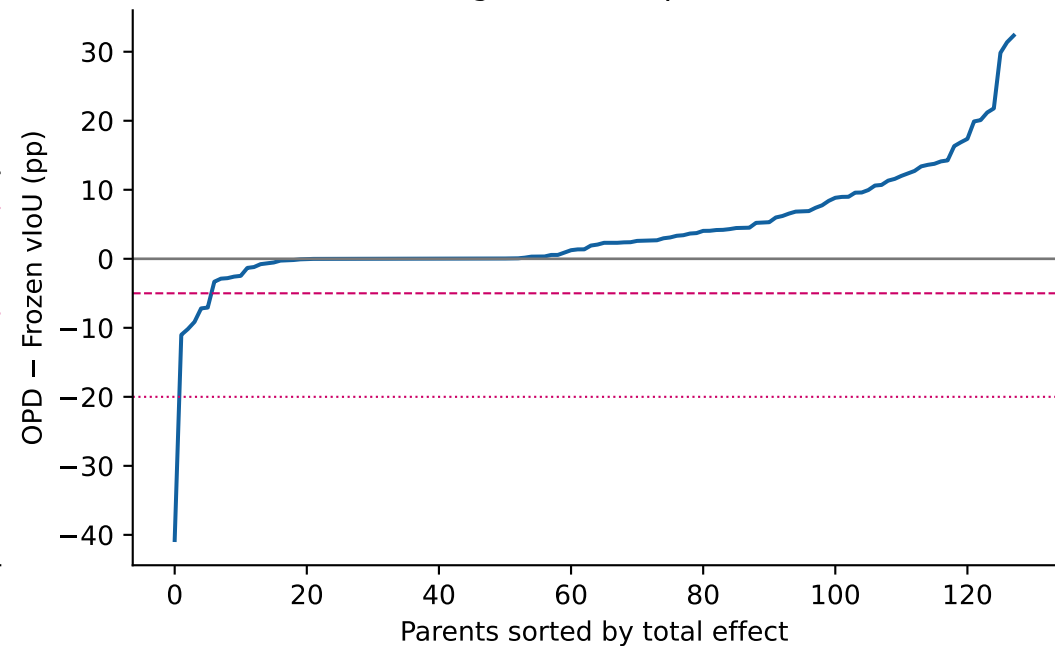
VidSTG target: all 128 parent effects
