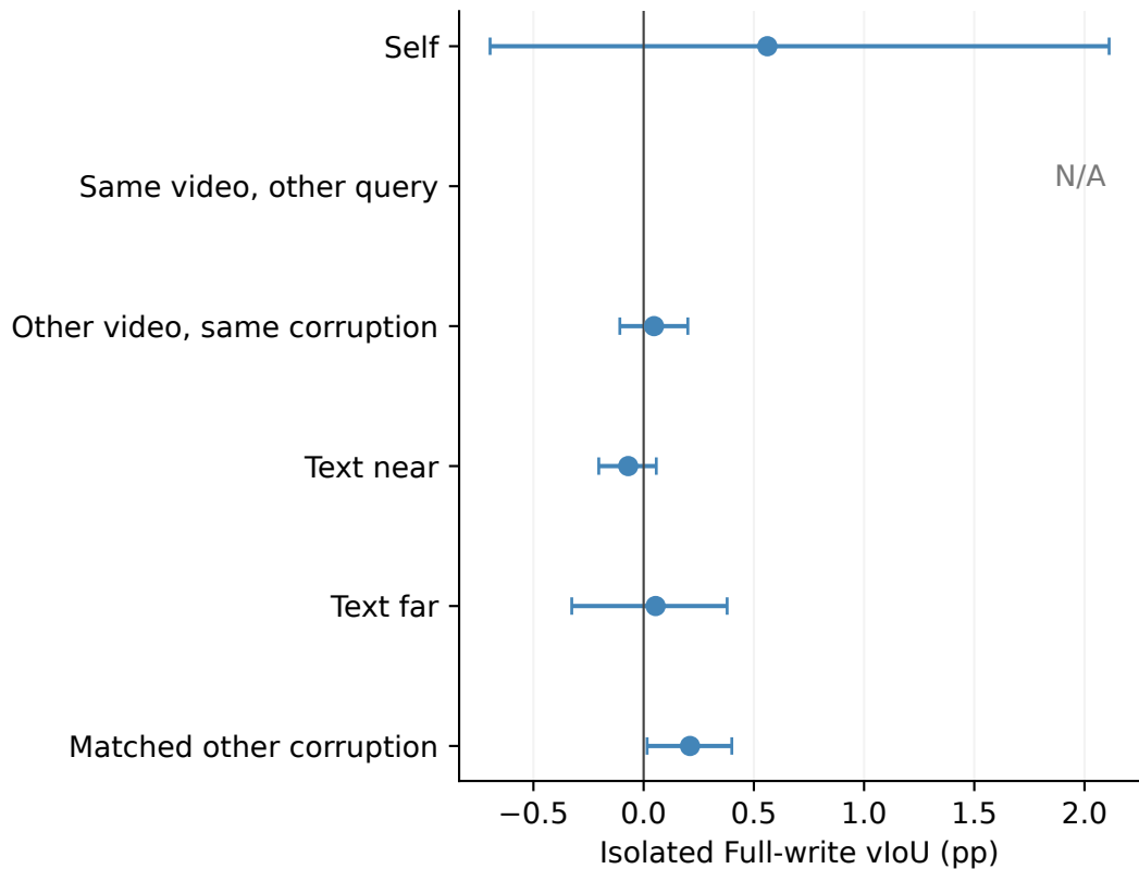
hc2 confirmation
