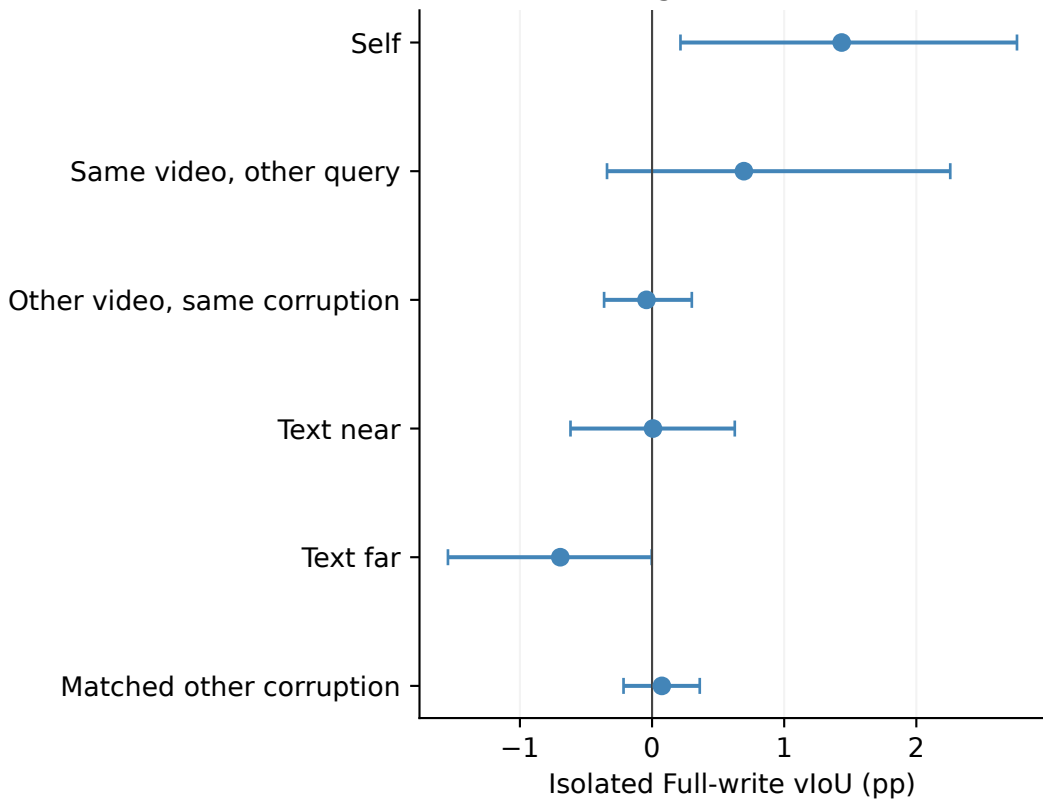
vidstg confirmation
