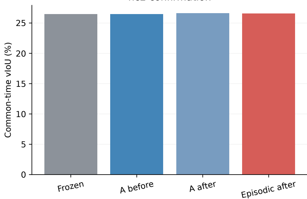
hc2 confirmation
