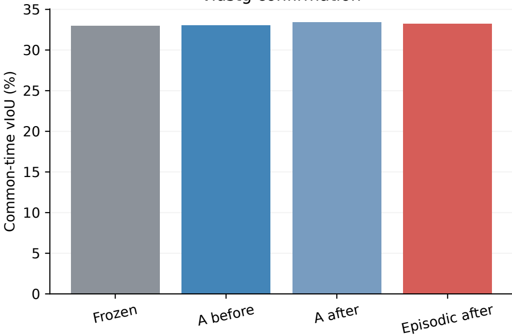
vidstg confirmation
