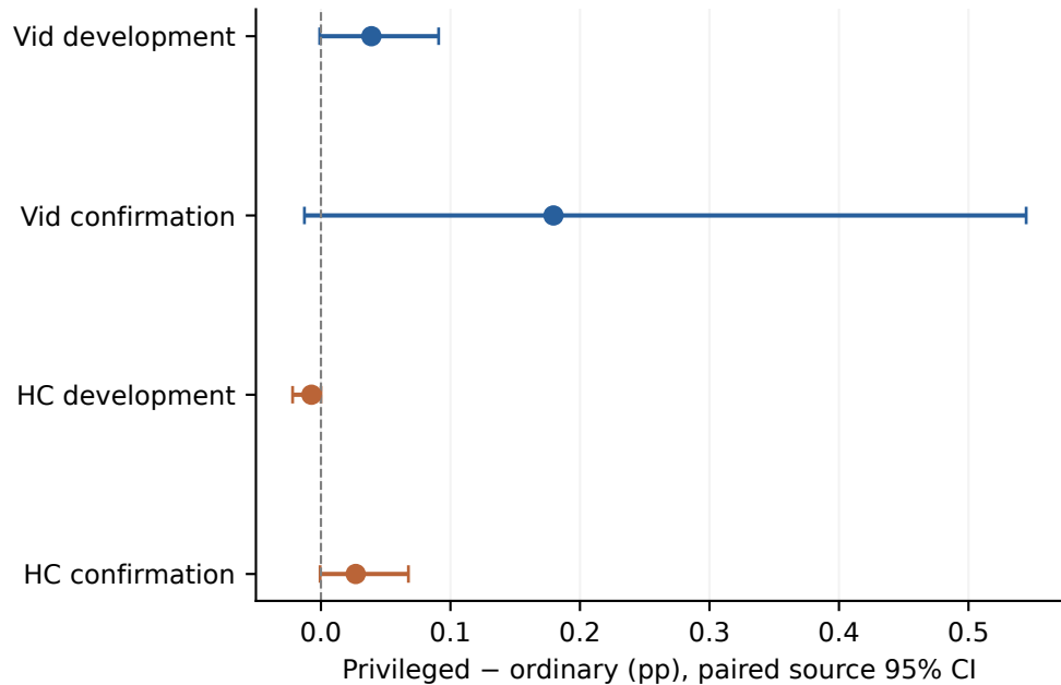
Full-tube vIoU
