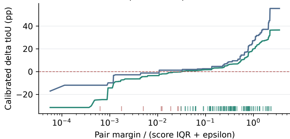
VidSTG | Pair-Norm | 31 sources
