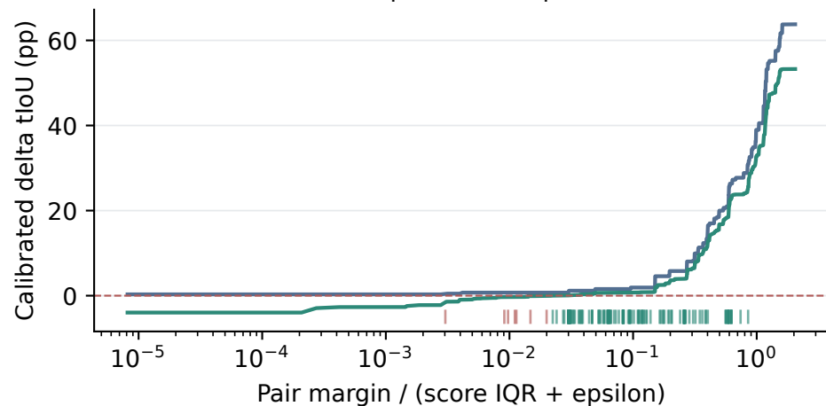
HC-STVG-v2 | Pair-Norm | 16 sources
