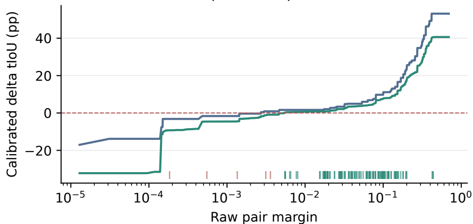
VidSTG | Pair-Raw | 31 sources
