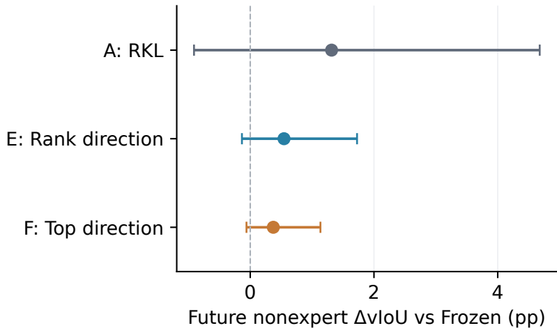
HC-STVG-v2
