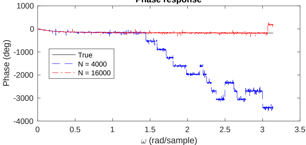
Phase response
