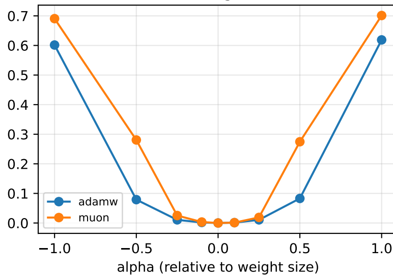
(h) loss increase along random directions
