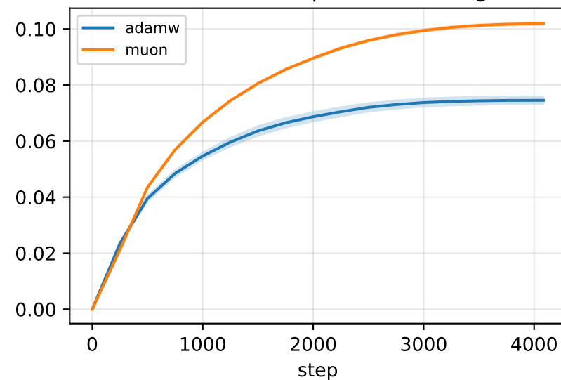
(c) distance from pretrained weights
