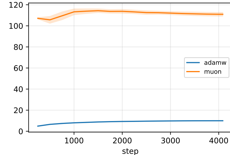
(f) stable rank of W - W_0
