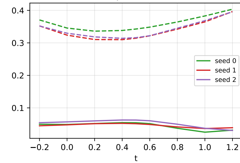
(i) AdamW ( t=0 ) to Muon ( t=1 ) solid: train probe, dashed: test
