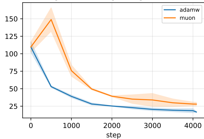
(g) Hessian largest eigenvalue
