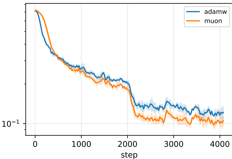
(a) train loss
