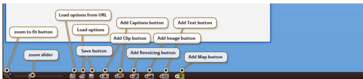
Figure 9. The Container Toolbar
