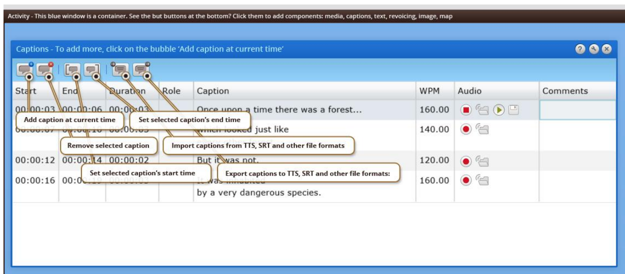
Figure 15. The Captions/Revoicing Component Toolbar
