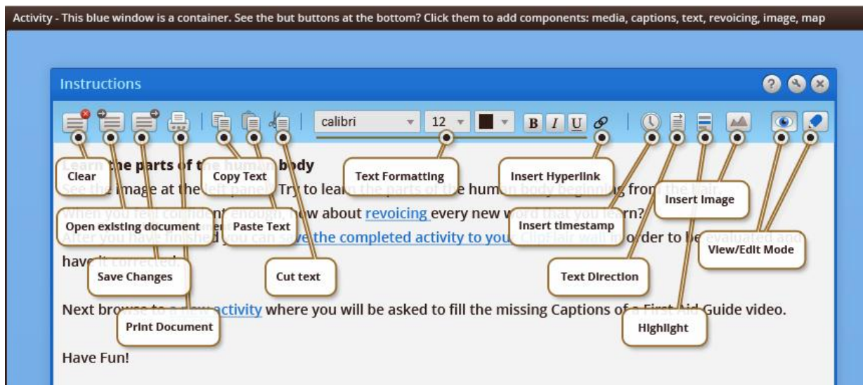
Figure 20. Text Component Toolbar
