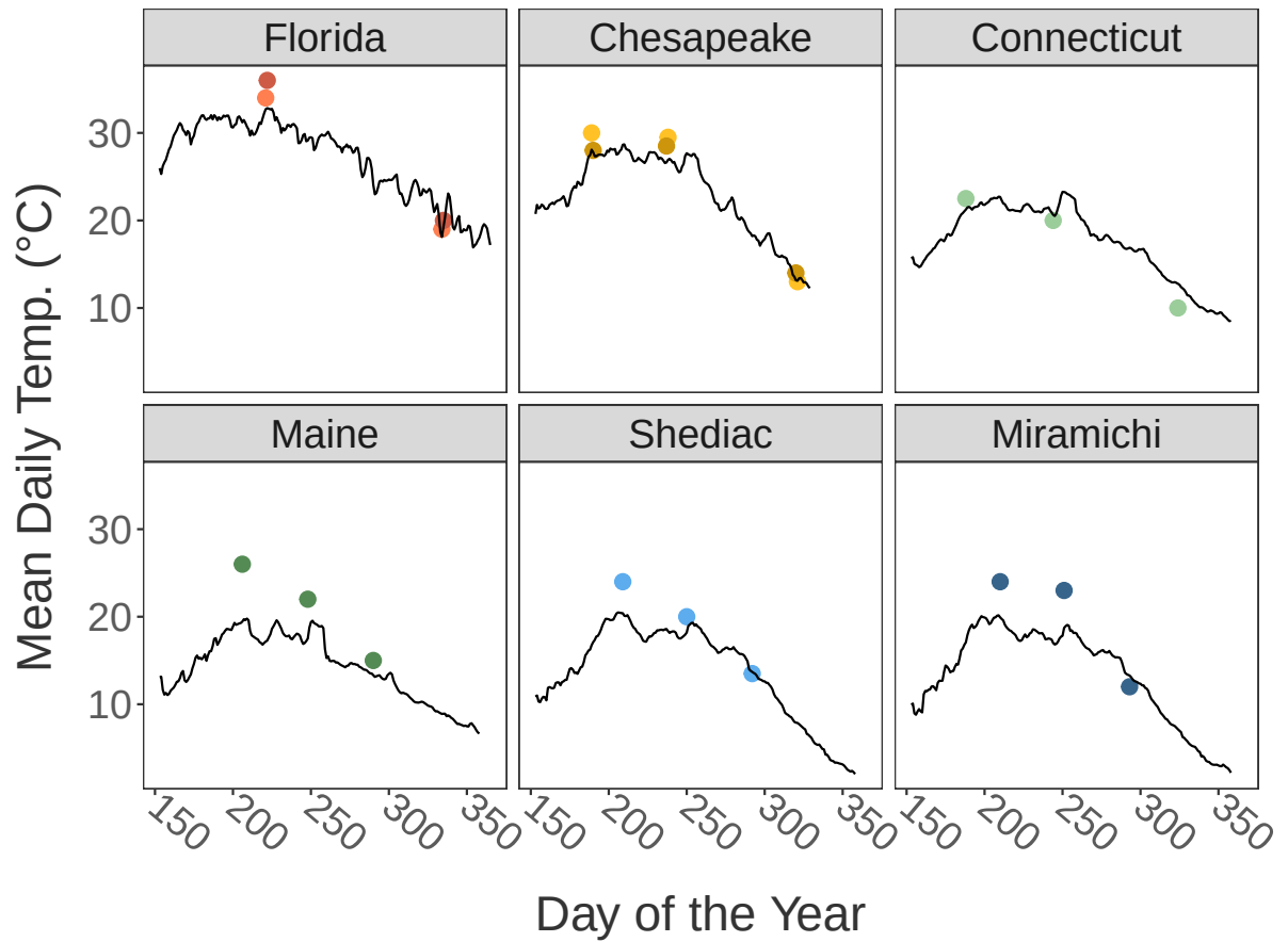
Figure S1: Continuous temperature profiles for the regions. These temperature profiles are shown with the temperatures measured during the time of collection included for comparison. While collection temperatures in Maine did not always match the recorded daily averages, across all sites the temperature records do give a general sense of the timing of seasonal maxima (and the proximity of collections to the seasonal maximum temperature).
