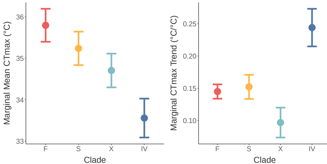
Figure 6: Clade marginal means (i.e. genetic variation in thermal limit) and the marginal trend (i.e. combined effect of local adaptation and plasticity).
