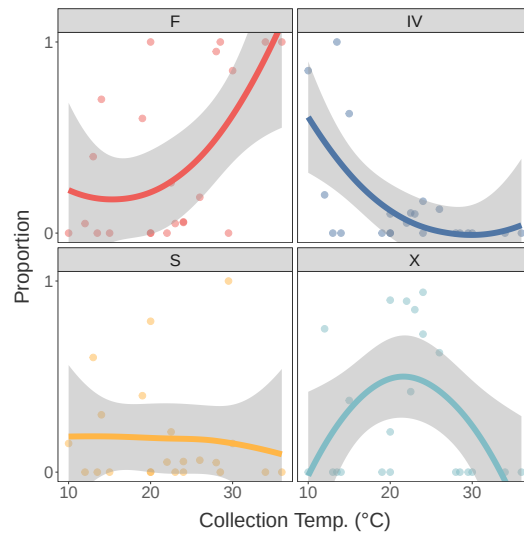
Figure 4: Clade proportions in each sample vs. collection temp.
