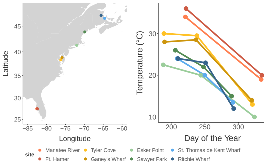
Figure 1: Map of sites (A) and collection temperatures recorded during each collection (B)
