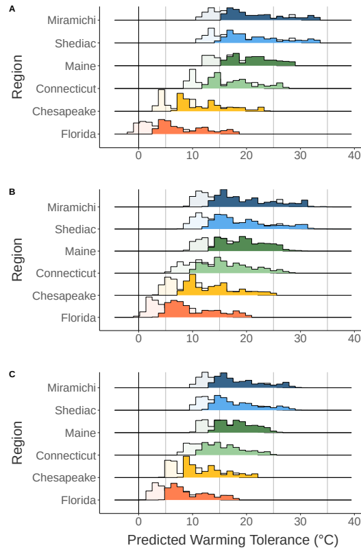
Figure 7: Warming tolerance during the peak season for each region, estimated under three scenarios; 1) a fixed CTmax value across the entire range, 2) fixed CTmax estimates for each individual clade, and 3) clade-specific CTmax and temperature acclimation. Current estimates of warming tolerance are shown in solid bars, with the estimates assuming a 4°C future warming shown with the lighter bars.
