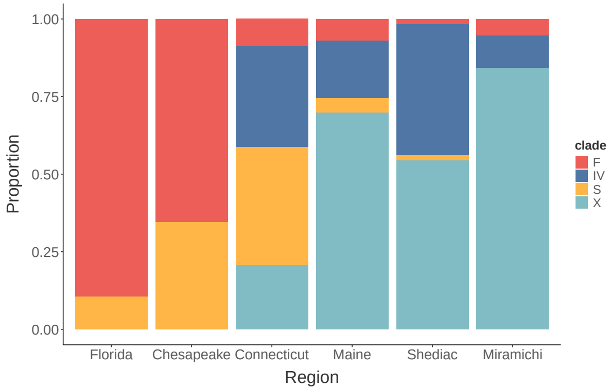
Figure S3: Observed proportions of the different clades in each region, as used in the simulated populations.
