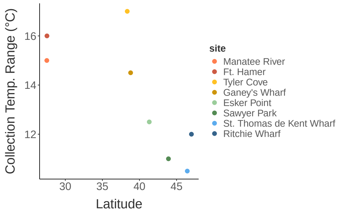
Figure S4: Collection temperature seasonality against latitude.
