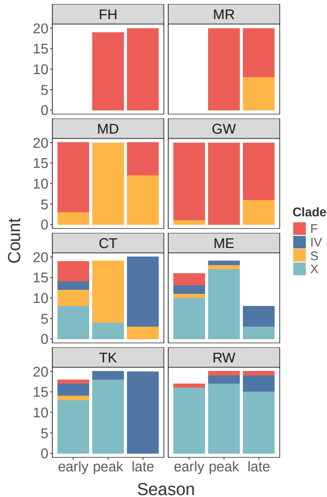
Figure 3: The distribution of clade identities at each site throughout the seasons. This plot includes just the 'high confidence' estimates - individuals identified as A. hudsonica were excluded, as were any individuals where less than 85% of the reads matched to any single clade)
