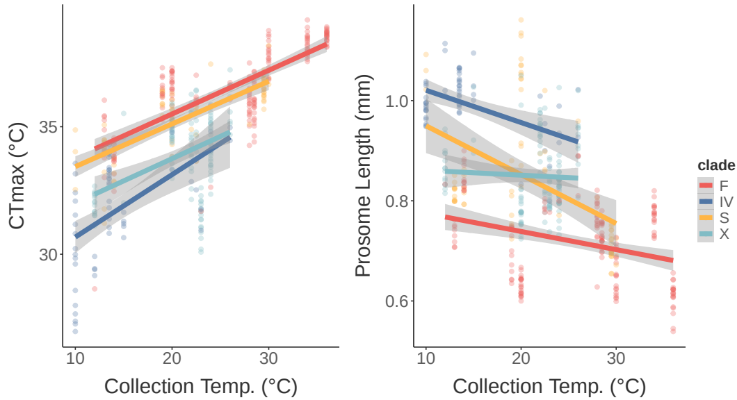
Figure 5: CTmax and body size vs. collection temperature, separated by clade.
