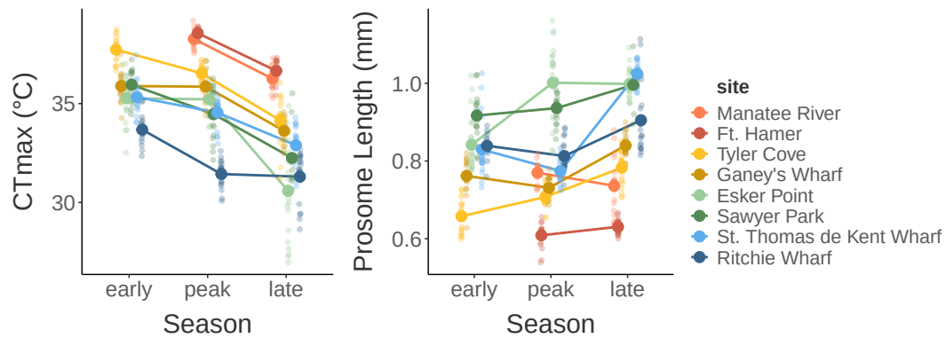
Figure 2: CTmax vs. season (A) and size vs. season (B) for each site
