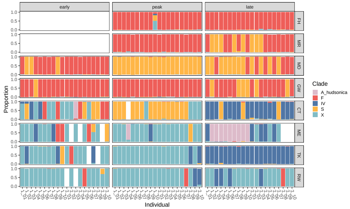
Figure S5: Individual clade prop plot (shows the proportion of reads for each individual that matched to the different clades)
