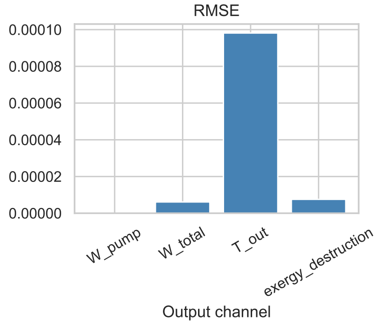
Physics-by-construction surrogate — held-out test set (10%)
