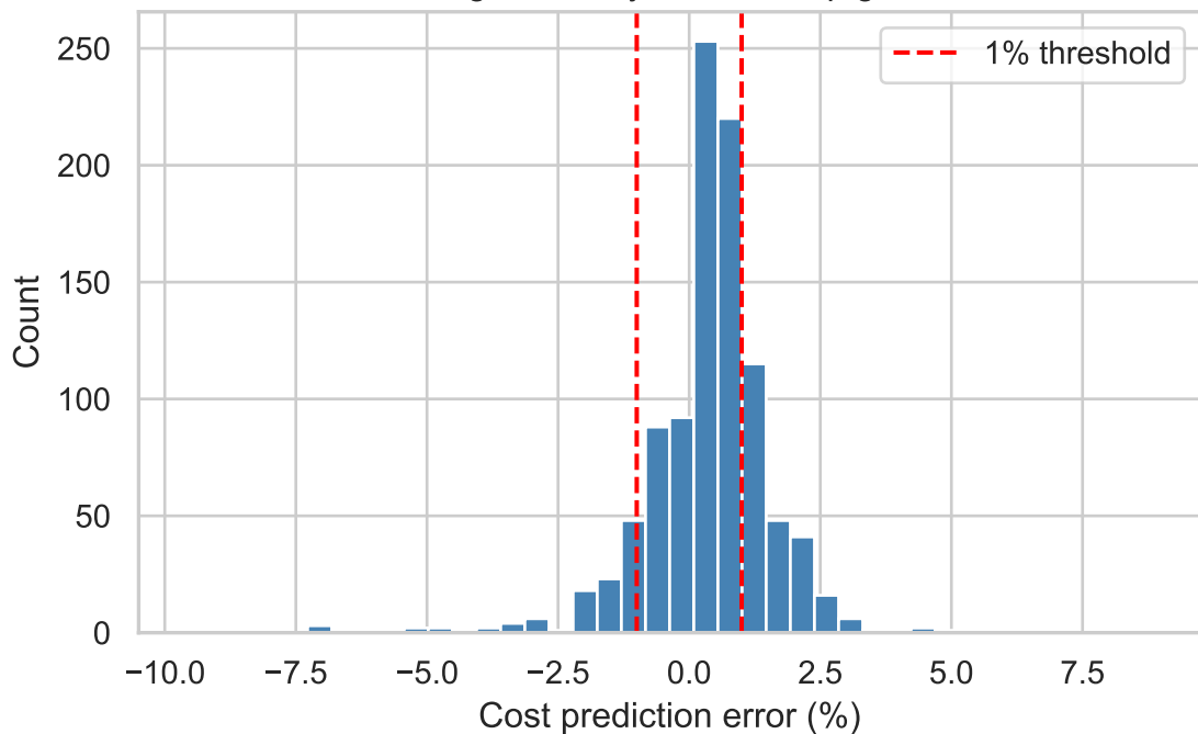
PINN surrogate fidelity vs CoolProp ground truth
