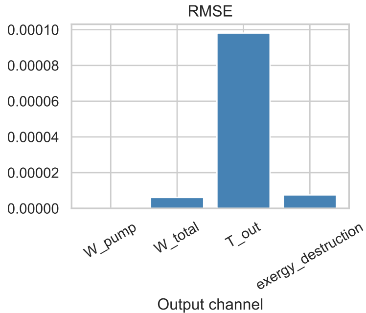
PINN surrogate — held-out test set (10%)
