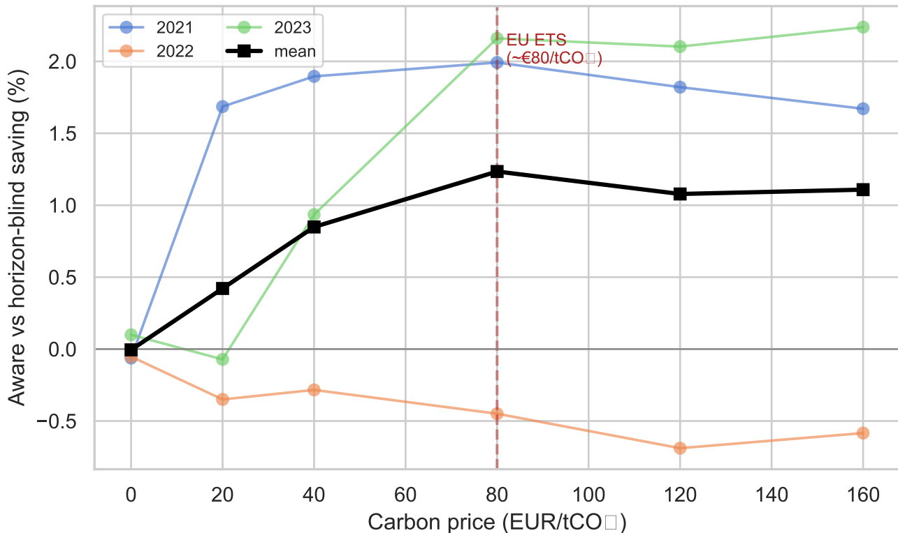
Composition-aware dispatch saving vs carbon price
