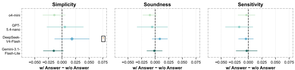
PRMBench
