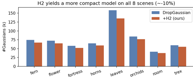
Fig. 1. Final Gaussian count, original vs. +H2. H2 produces a more compact model on all eight scenes ( \sim 10.7\% mean), a deterministic, noise-free effect.
