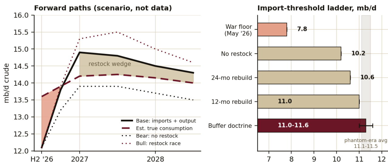
Figure 7. Left: forward paths for apparent demand against estimated true consumption; the shaded area is the projected restock wedge in the base case. Right: post-normalization import run-rates and what each implies. All values are scenario projections, not data.
