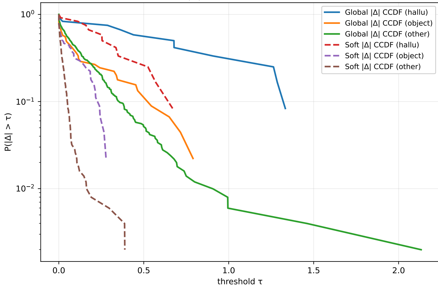
Token-level |\Delta| sparsity (CCDF) by token type
