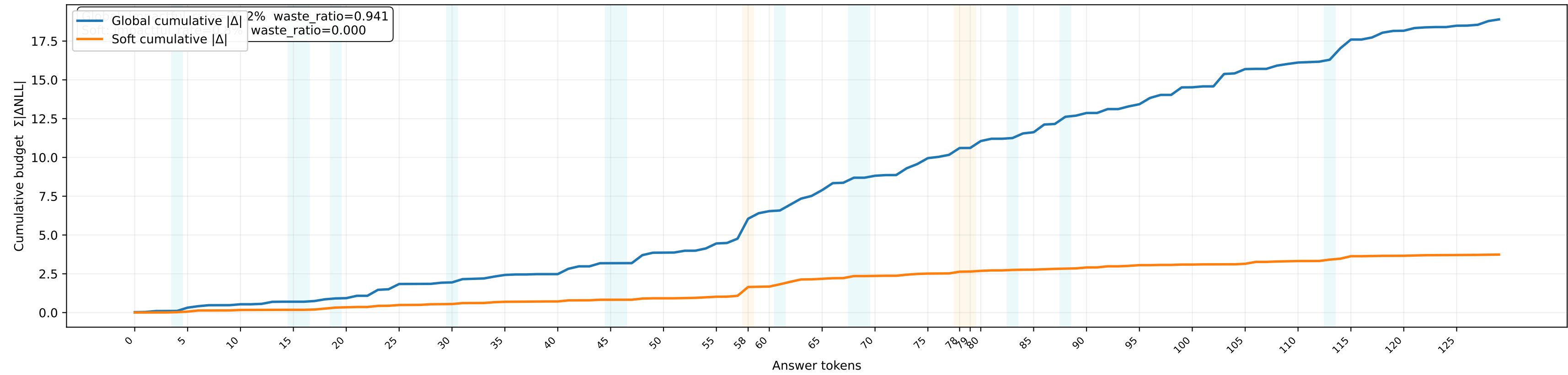
Scheme: Cumulative budget | case 75 (rank 0005)
