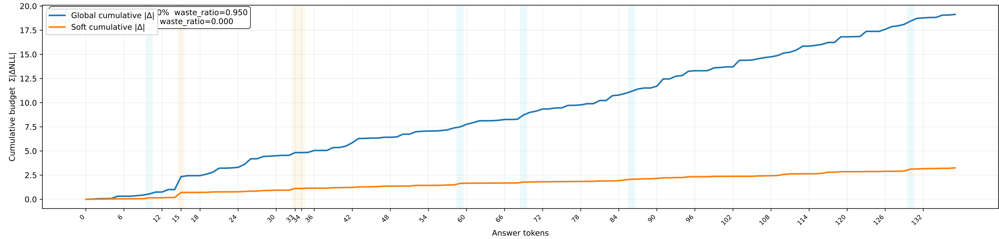
Scheme: Cumulative budget | Case 15 (rank 6664)
