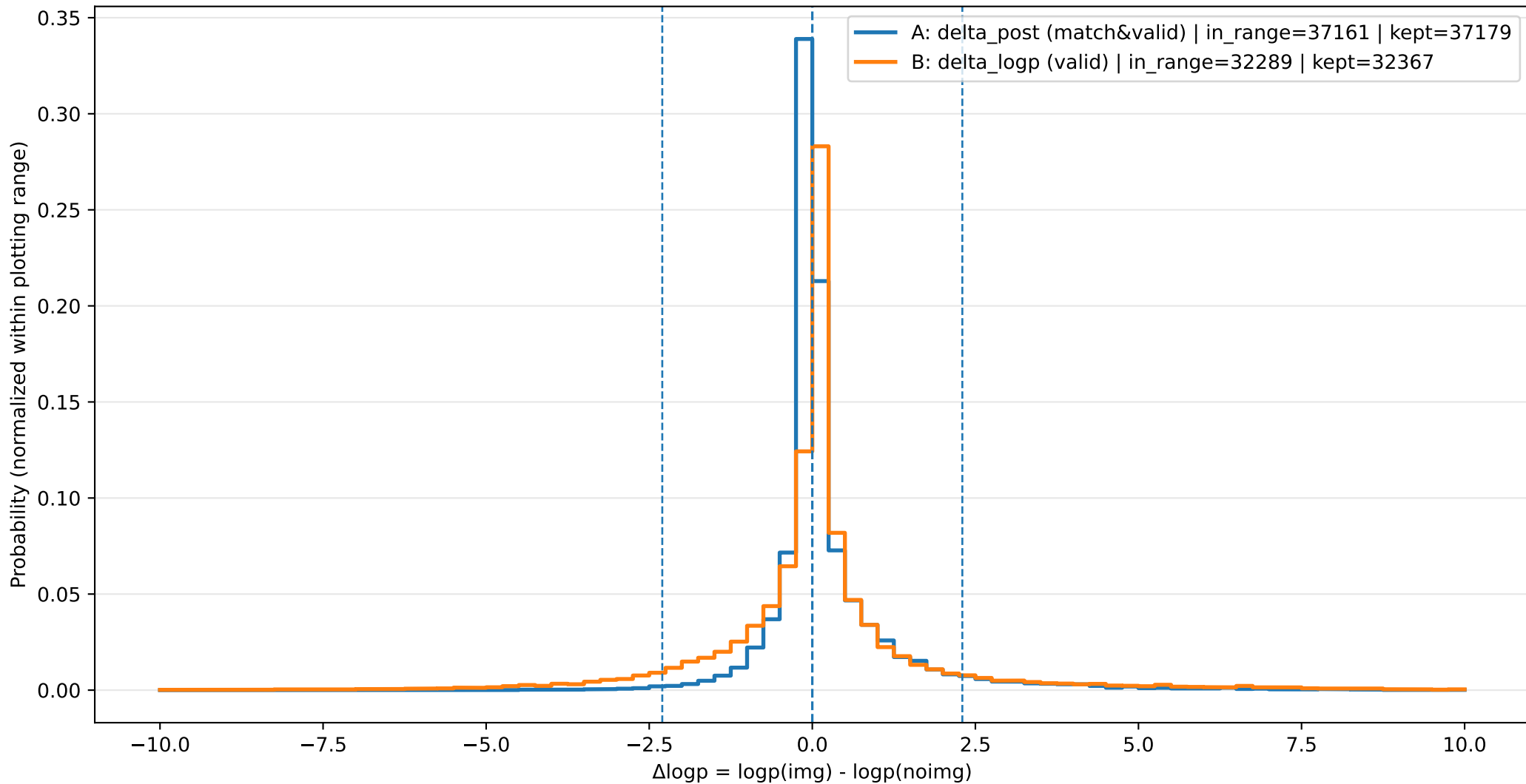
Delta Distribution Overlay (bin=0.25, range=[-10.0,10.0))
