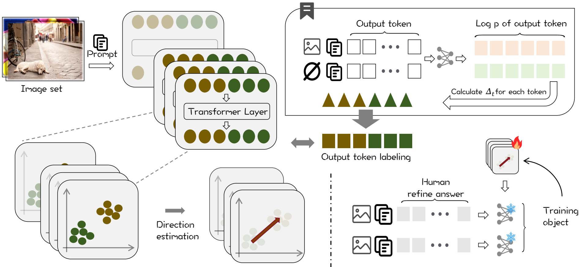
(1) Token-level extraction of steering vectors
