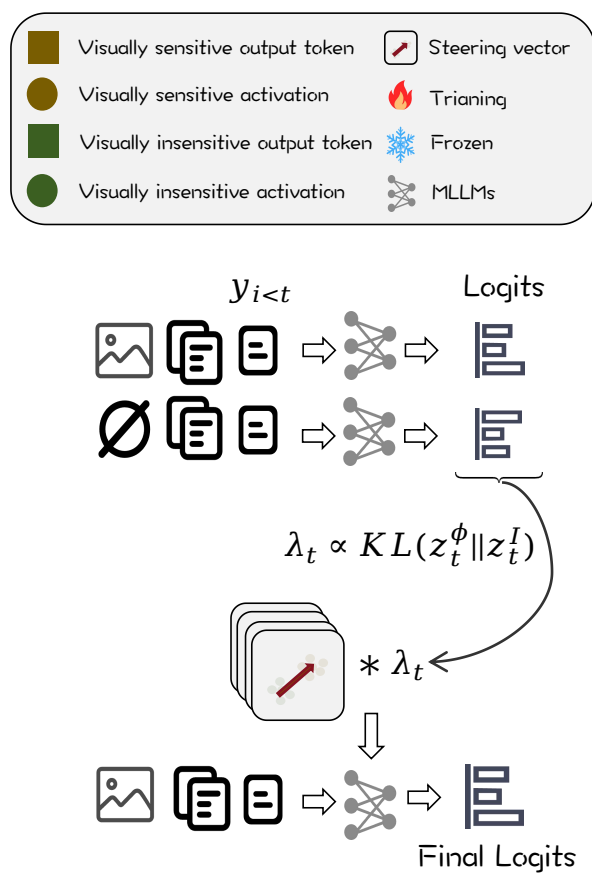
(3) Token-level adaptive steering
